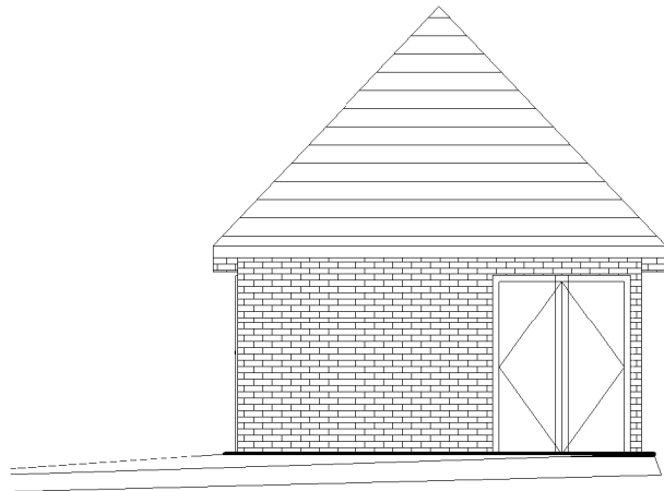
1 Existing Rear Elevation 1 : 100
