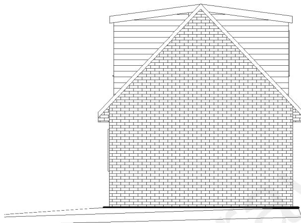
2 Proposed Rear Elevation 1 : 100
