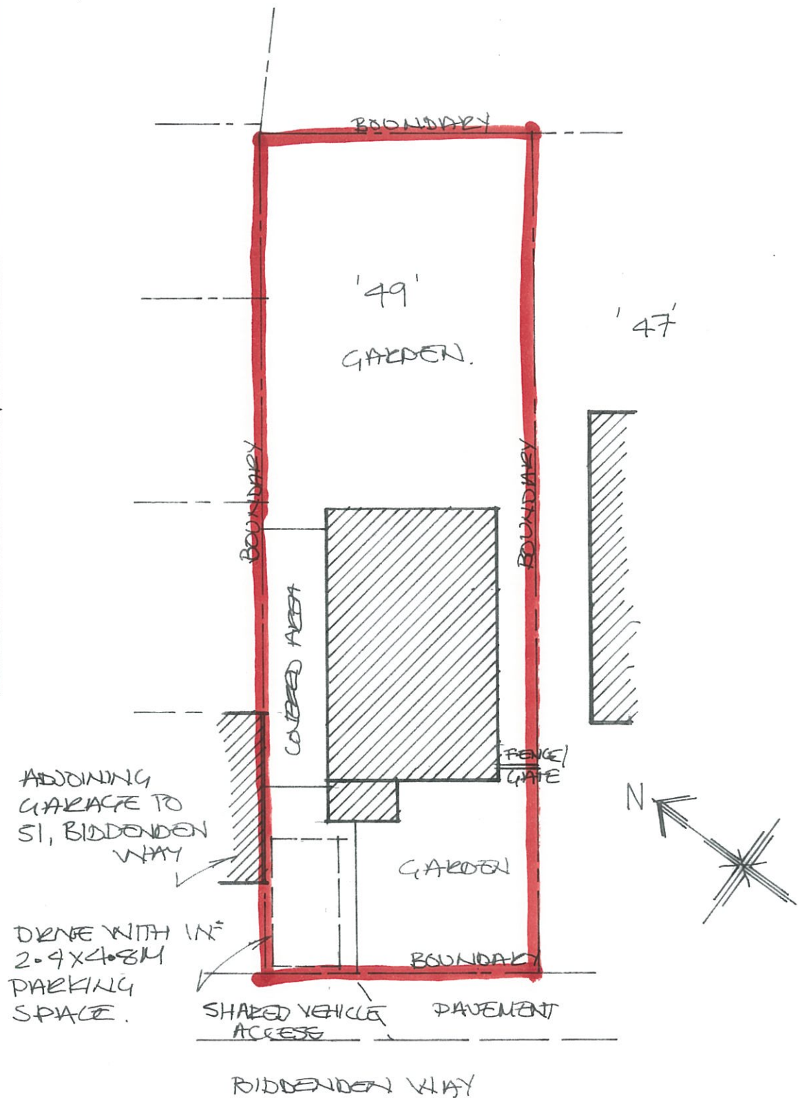
Exg. Block Plan.
