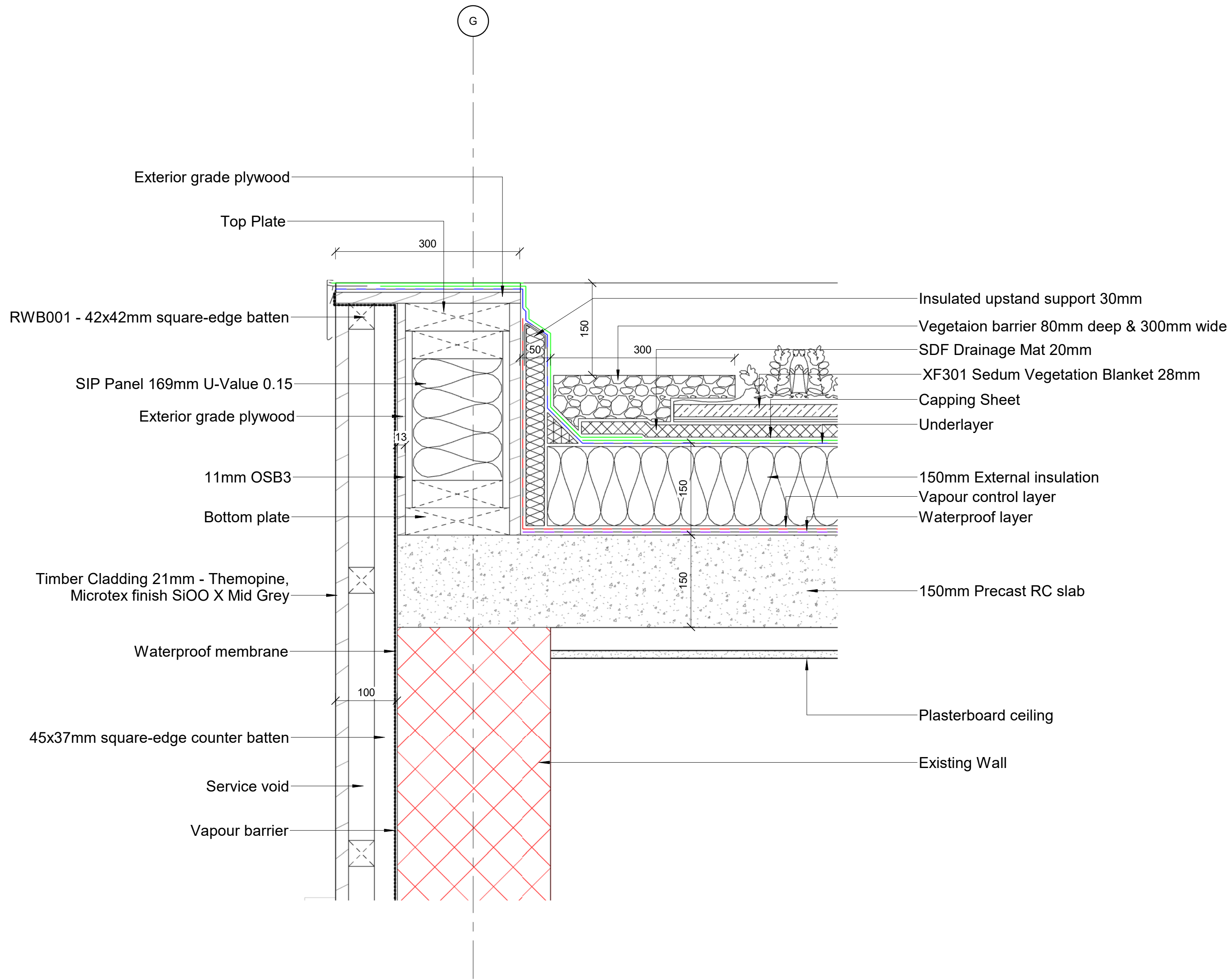
1 Roof Detail - Sedum Roof 27702 1 : 5
