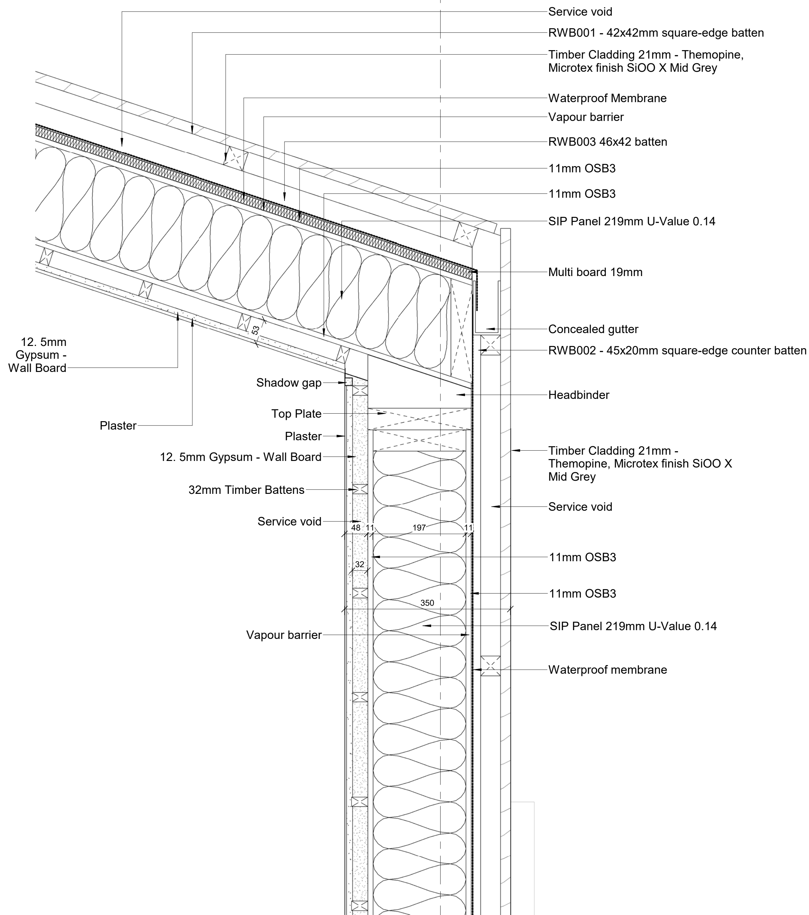
2 External Wall Detail - SIP B 1 : 5
