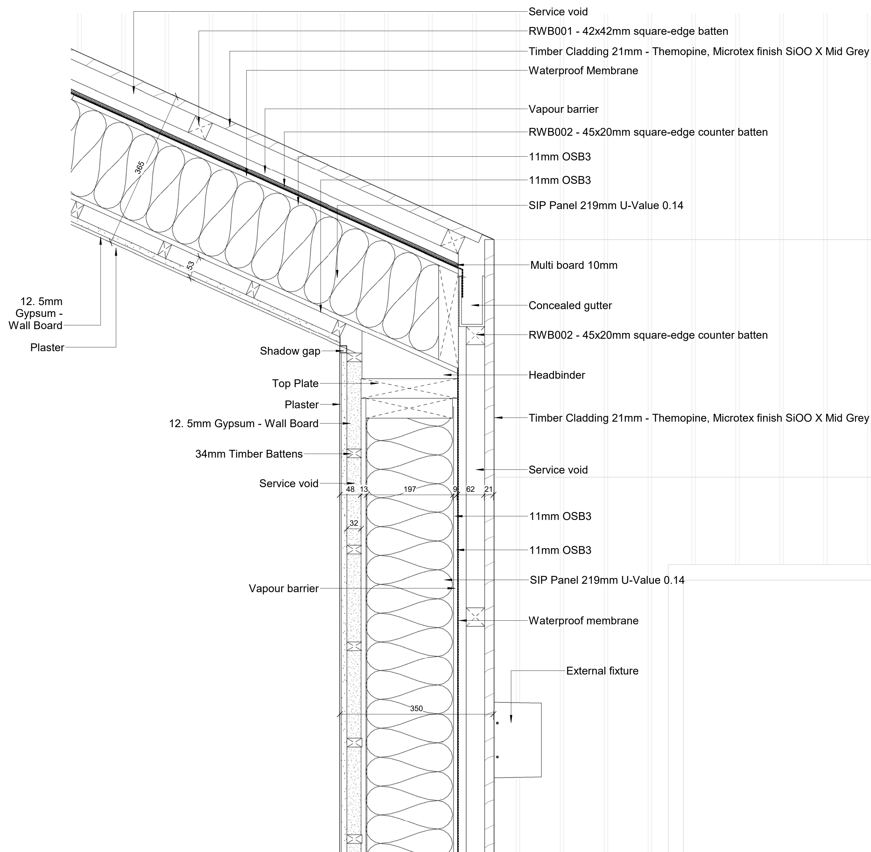
1 External Wall Detail - SIP A 1 : 5
