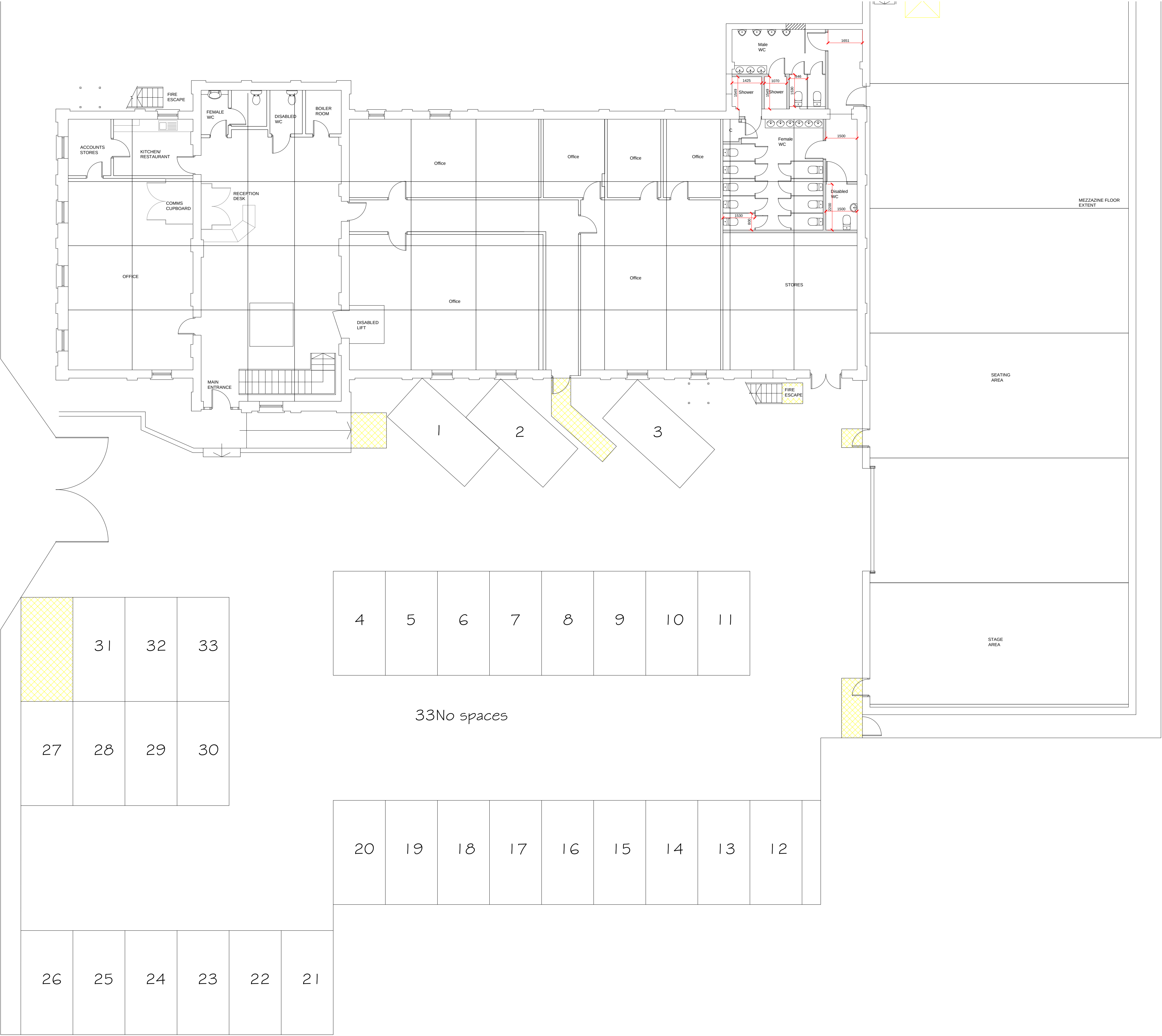
Proposed Parking Plan Scale 1:100
