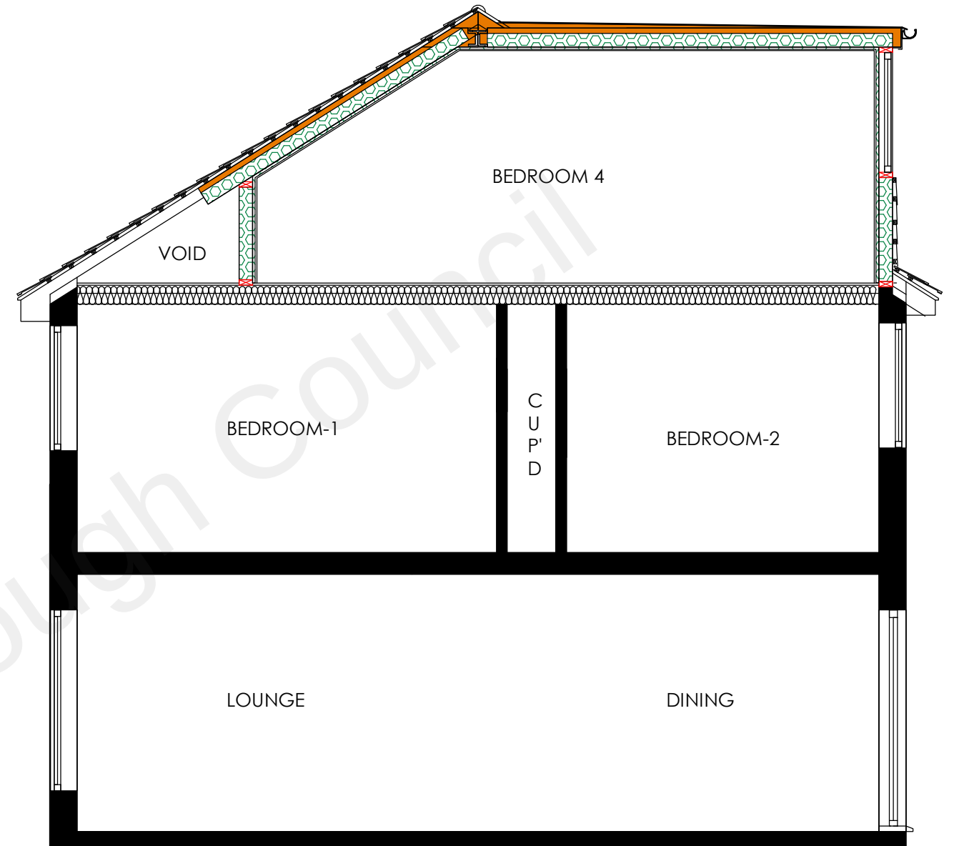
Proposed Cross Section AA 1 : 50
