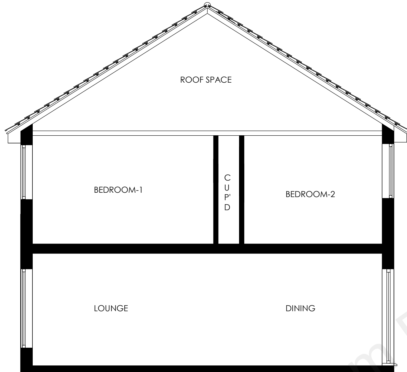
Existing Cross Section AA 1 : 50
