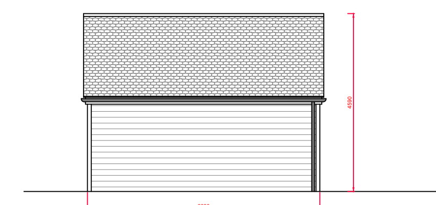
Side Elevation 1:100
