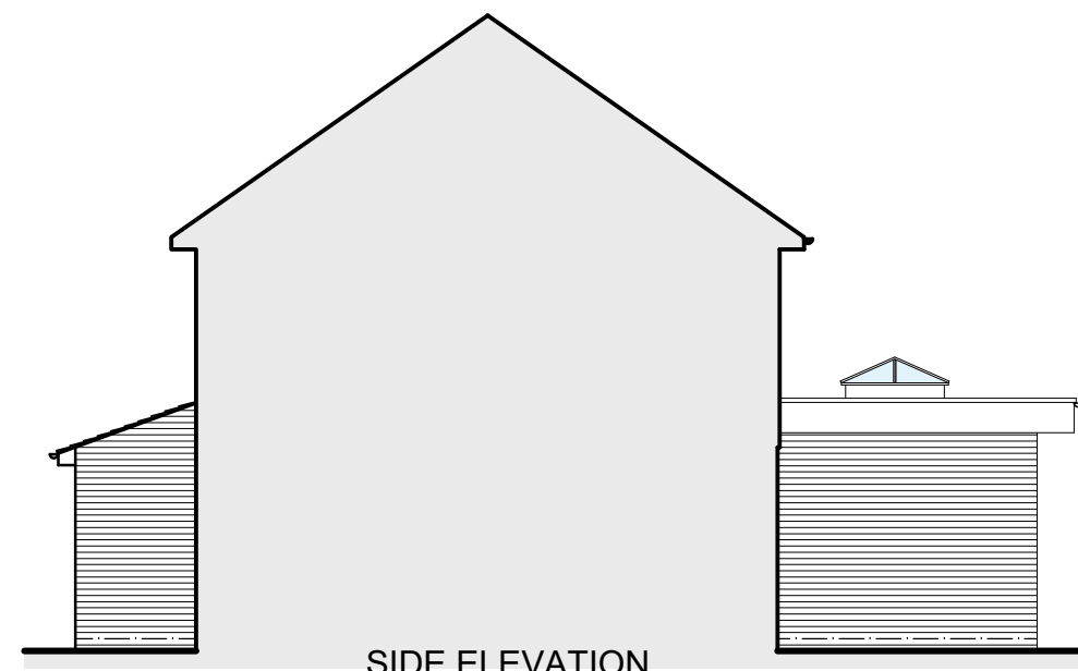
SIDE ELEVATION (1:100)
