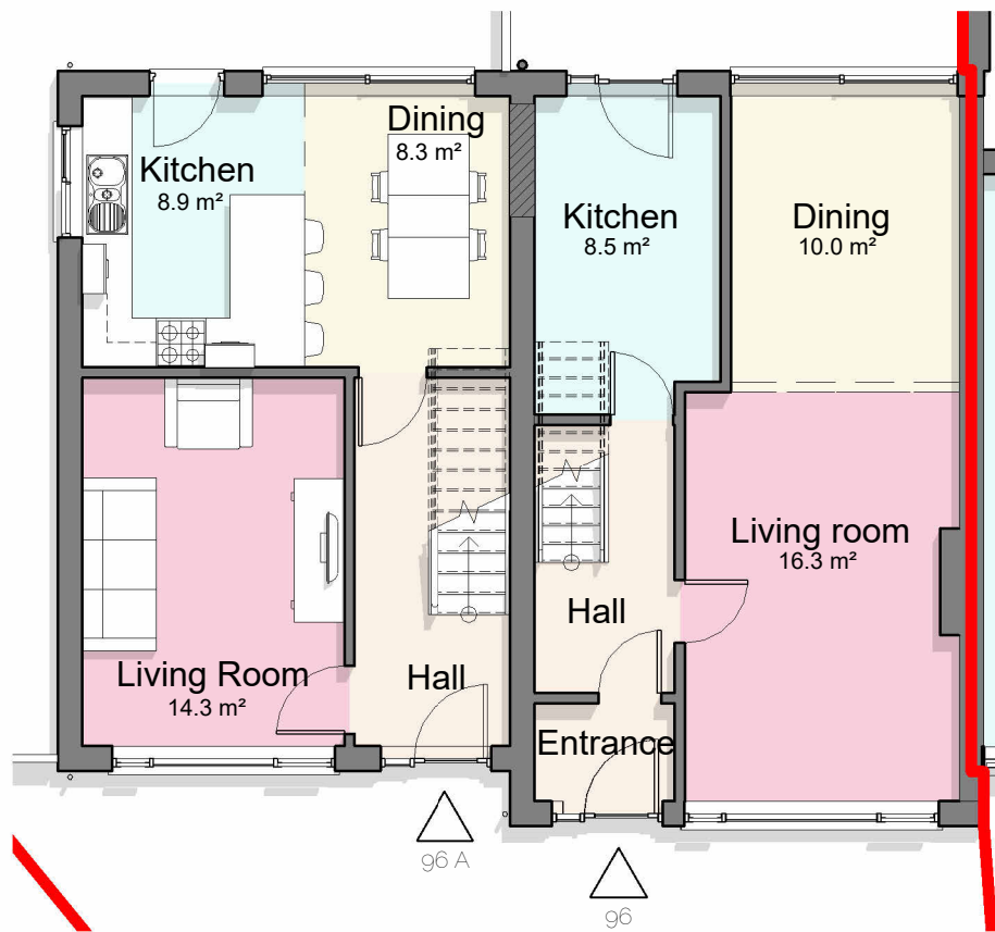
Proposed Ground Floor 1:100
