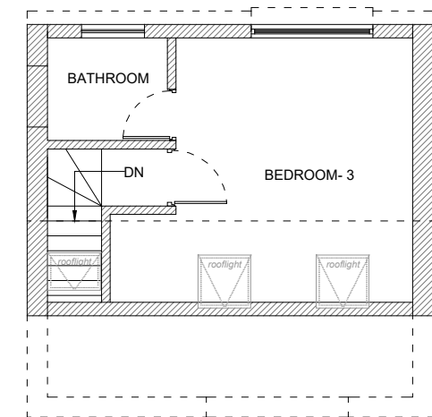
PROPOSED LOFT FLOOR PLAN
