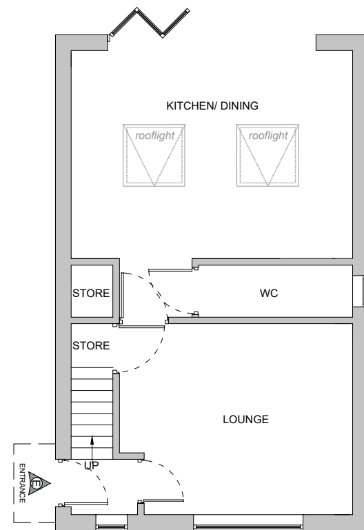
EXISTING GROUND FLOOR PLAN (no proposed changes)
