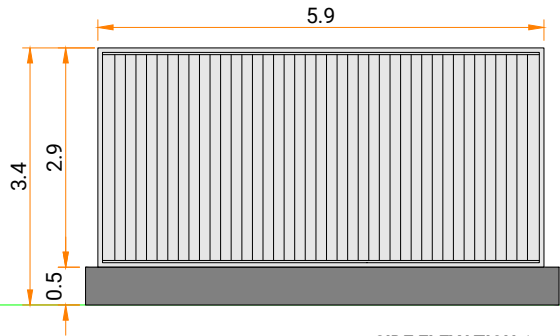
SIDE ELEVATION 1
