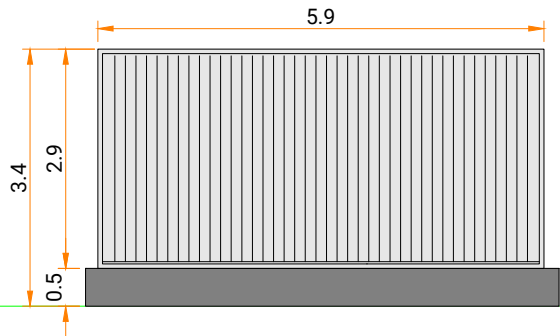
SIDE ELEVATION 2
