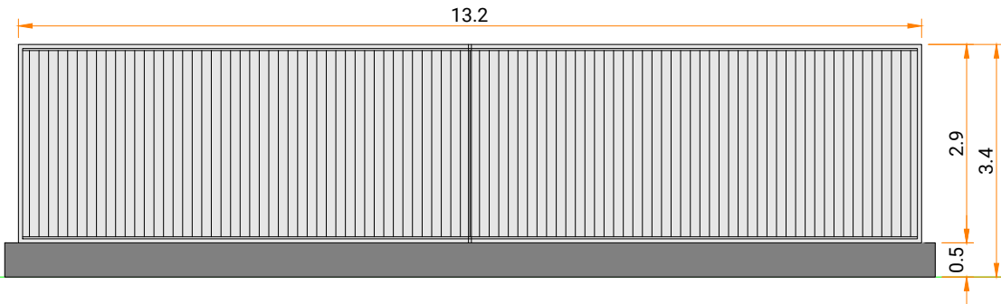
REAR ELEVATION
