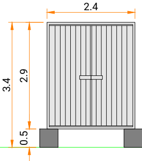
SIDE ELEVATION 1
