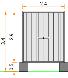
SIDE ELEVATION 2
