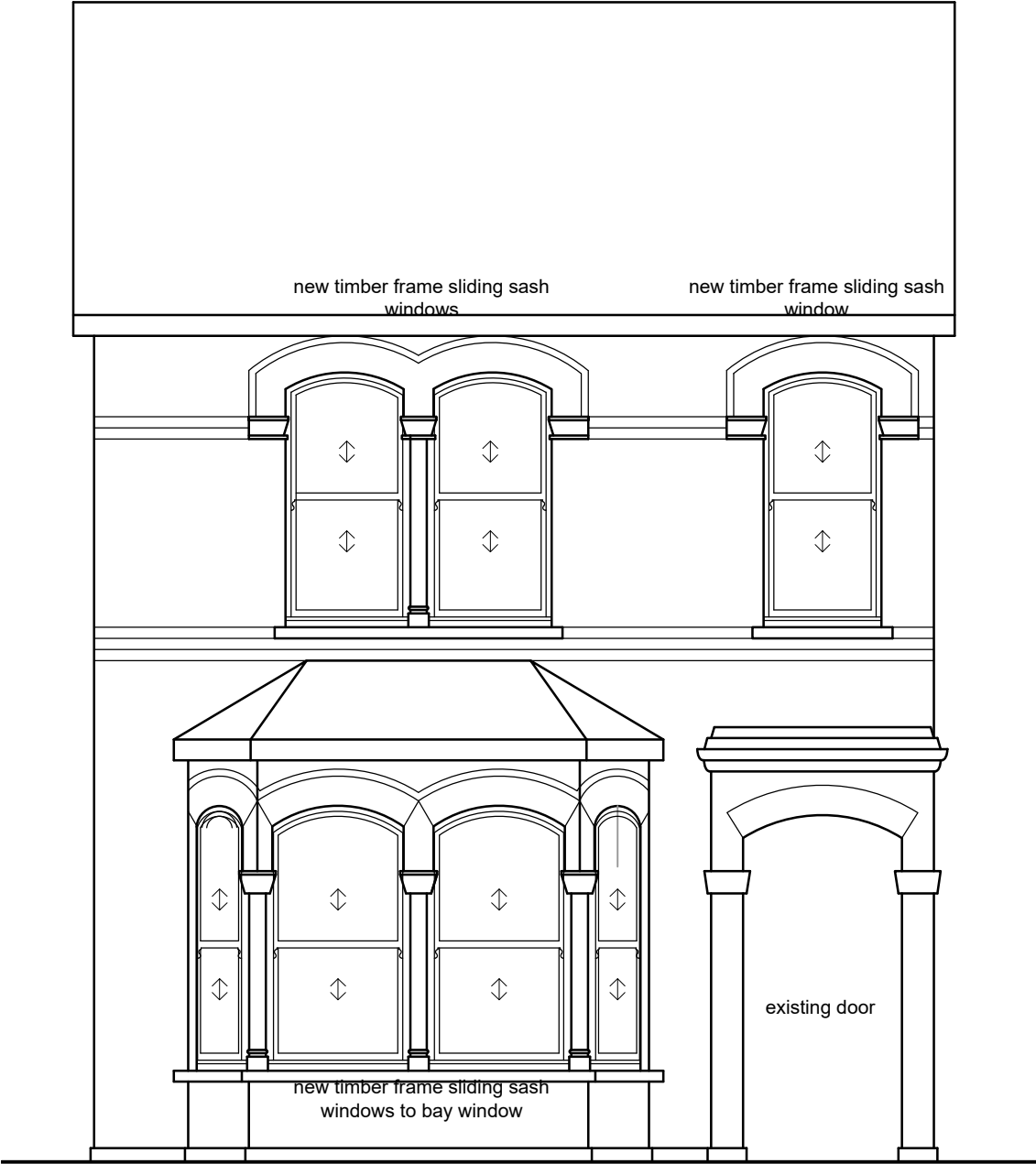
FRONT ELEVATION (1:50)
