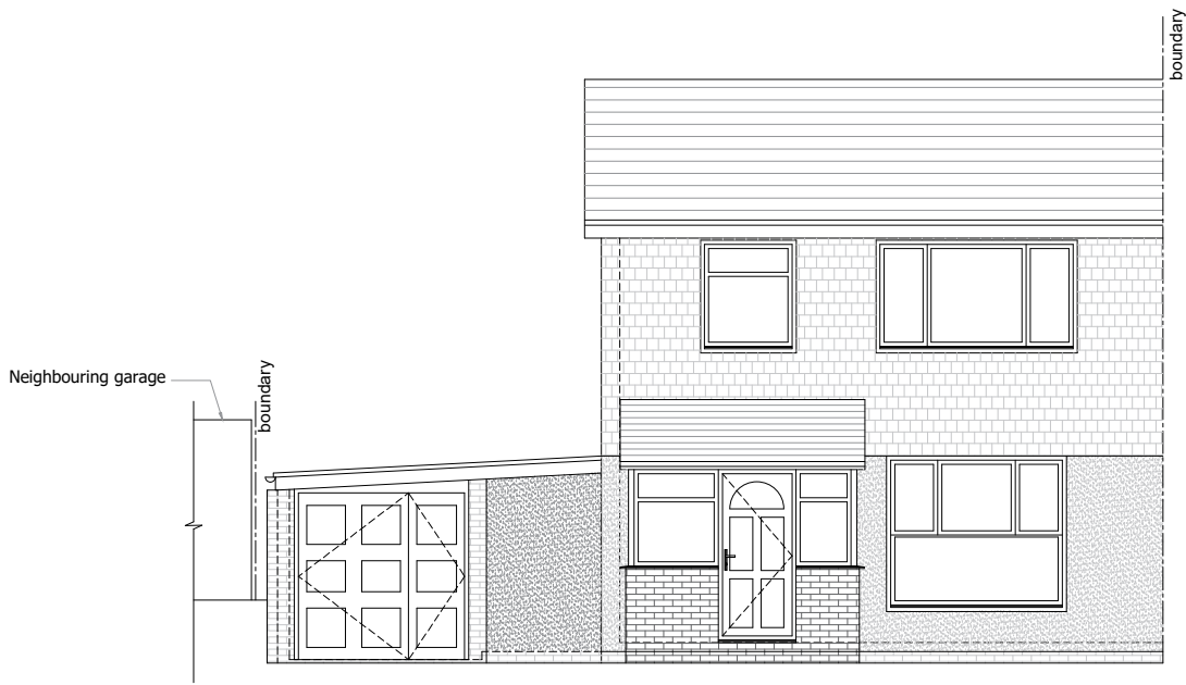
FRONT ELEVATION (Northerly facing)
