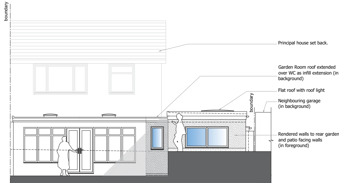
REAR ELEVATION (Southerly facing)
