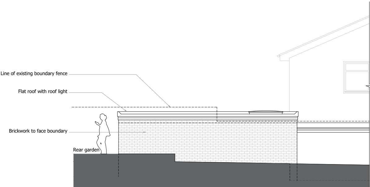
SIDE ELEVATION (Easterly facing)
