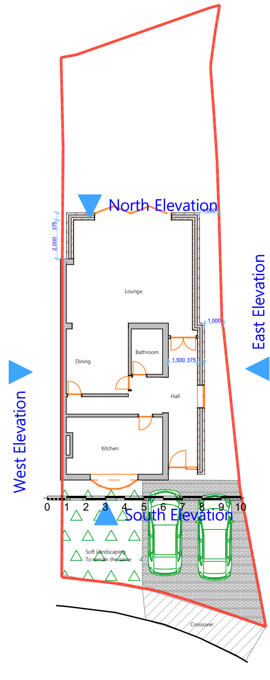
3 Site Plan Proposed 1:200
