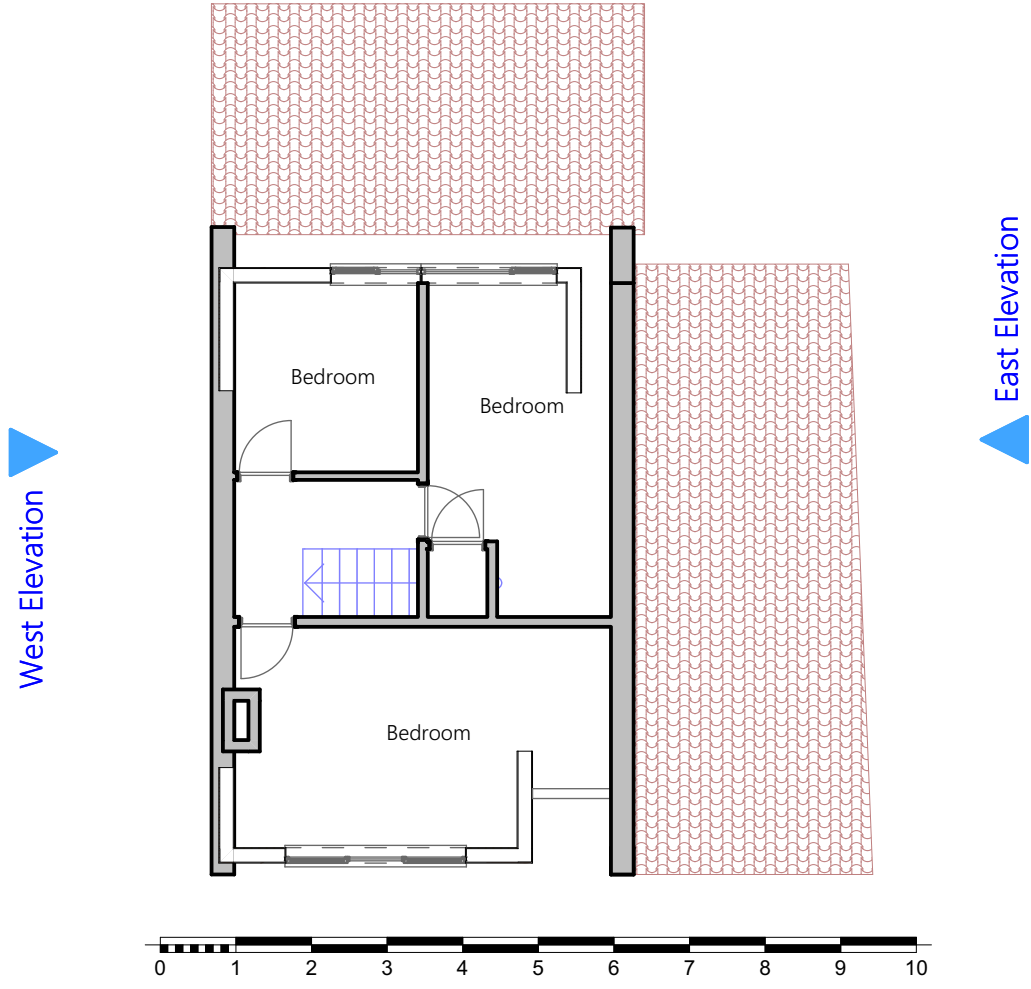
6 01 First Floor Existing 1:100
