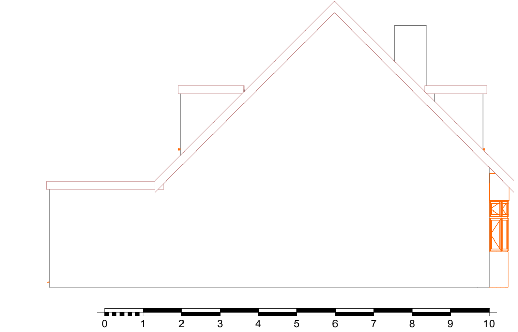
2 West Elevation Existing 1:100
