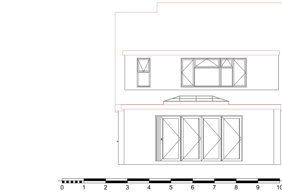
10 North Elevation Proposed 1:100
