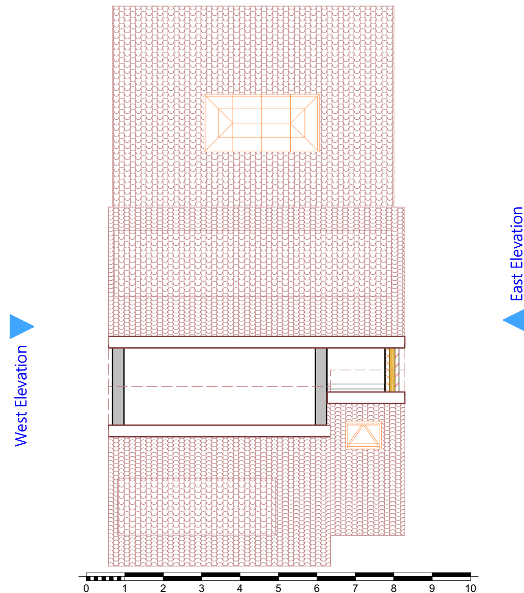
14 Roof Proposed 1:100
