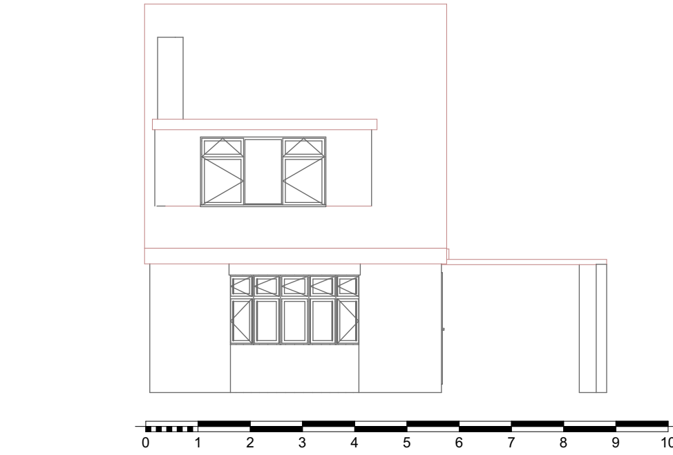
4 South Elevation Existing 1:100
