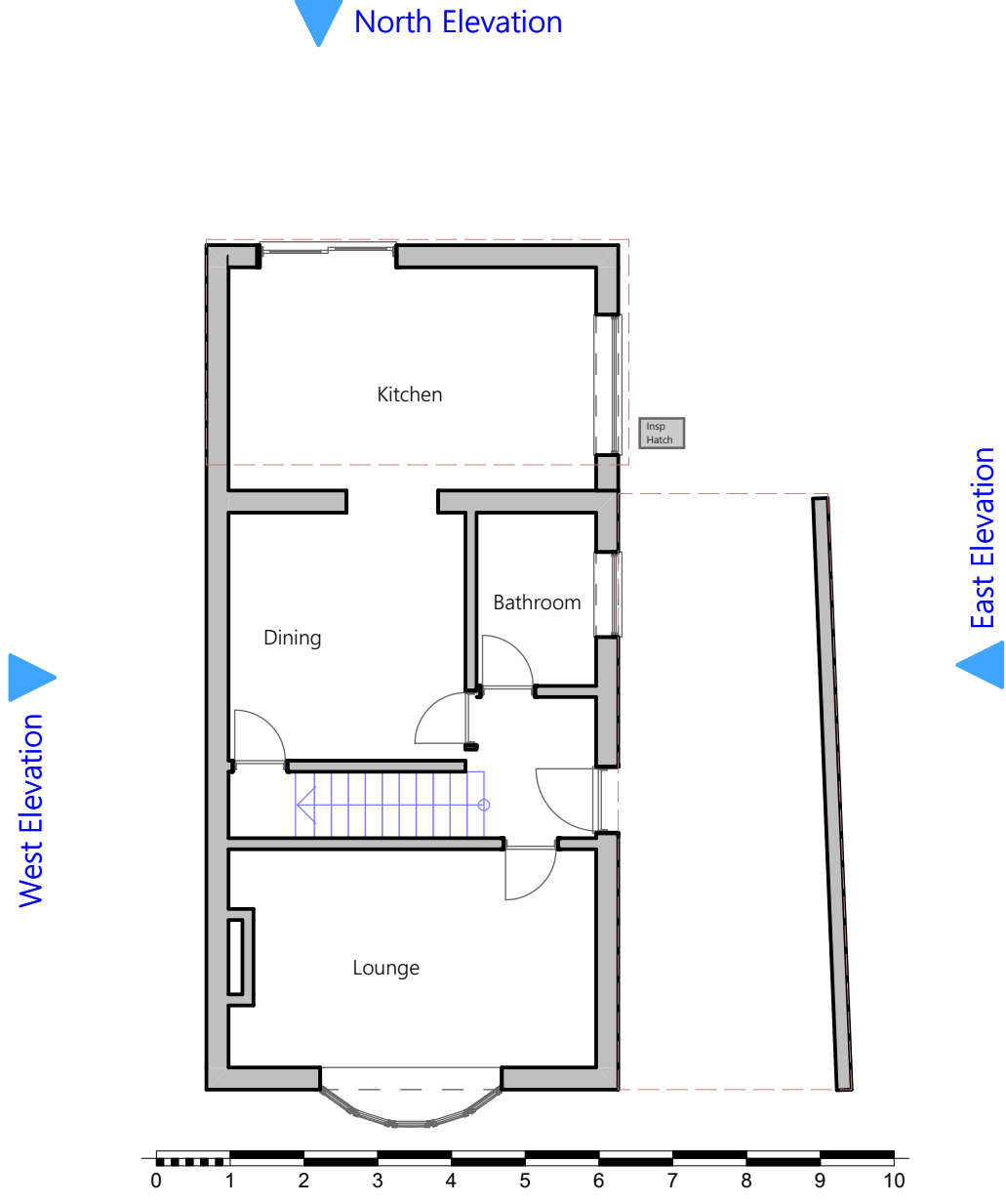
5 GF Ground Floor Existing 1:100
