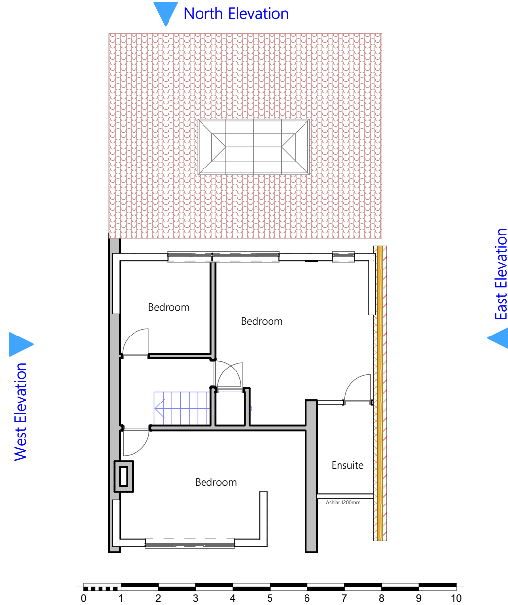
13 01 First Floor Proposed 1:100
