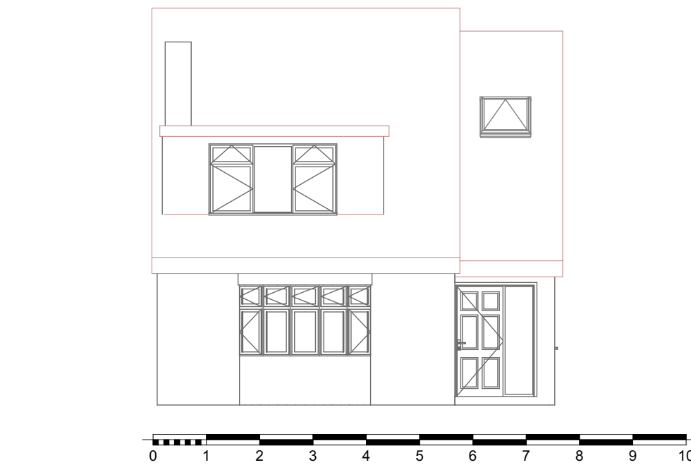
11 South Elevation Proposed 1:100
