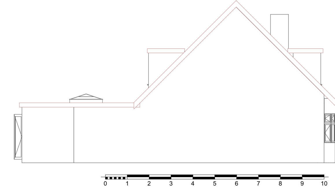
9 West Elevation Proposed 1:100
