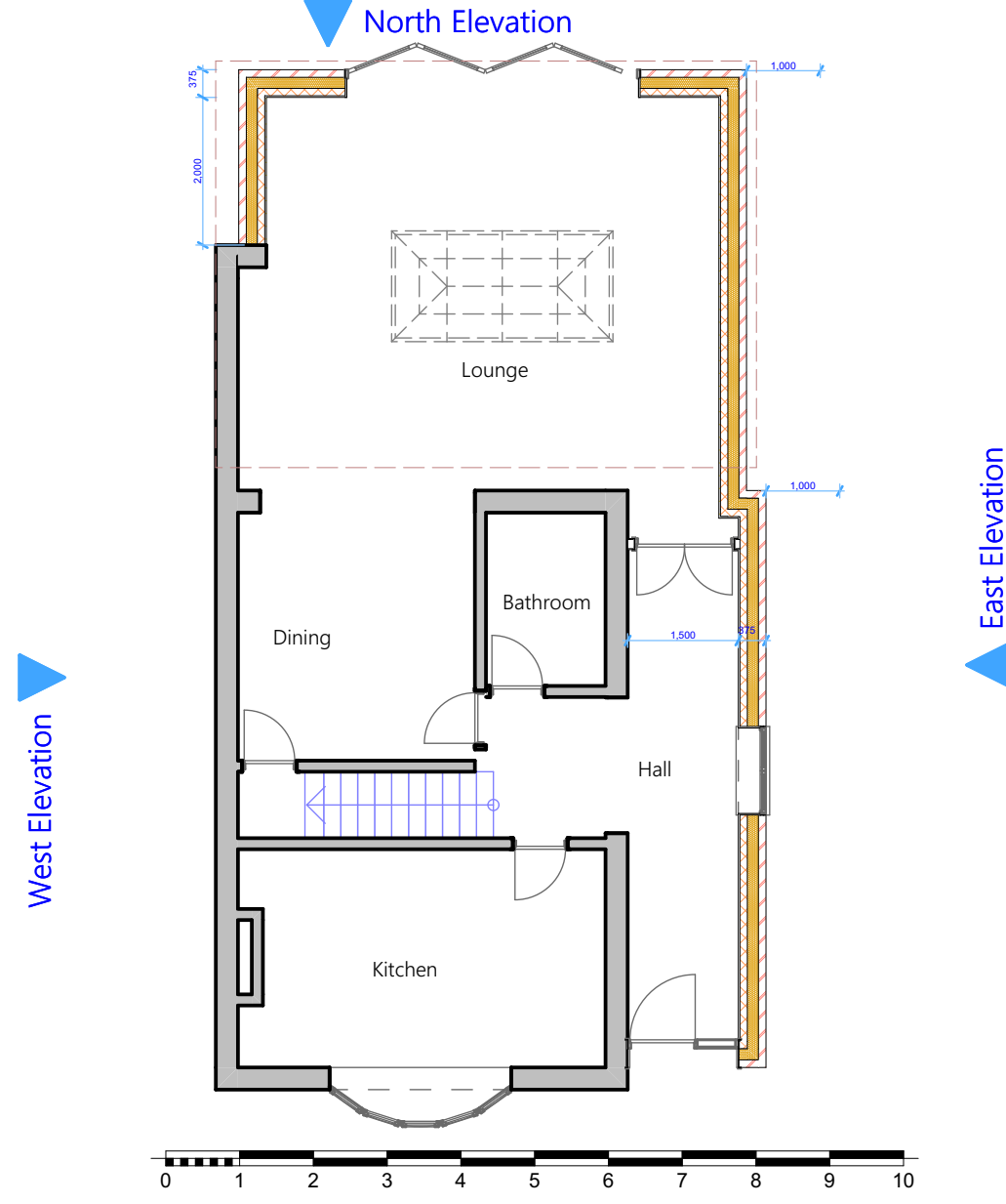
12 GF Ground Floor Proposed 1:100
