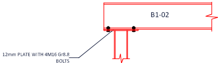
DETAIL A COLUMN HEAD
