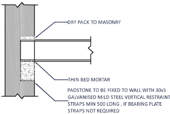
DETAIL B PADSTONE DETAIL
