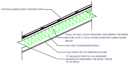
DETAIL C GARAGE ROOF BUILD UP
