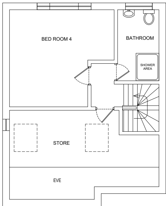
PROPOSED SECOND FLOOR / LOFT PLAN
