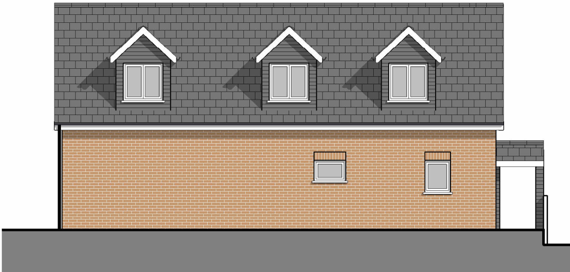
Existing and Proposed West Elevation 1 : 100
