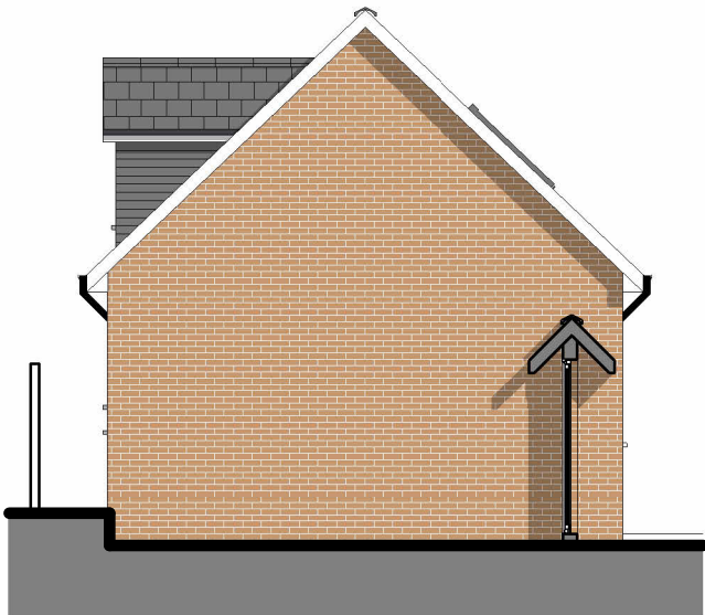
Existing and Proposed South Elevation 1 : 100
