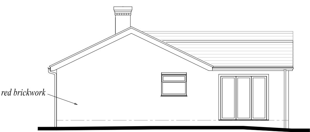
SIDE ELEVATION
