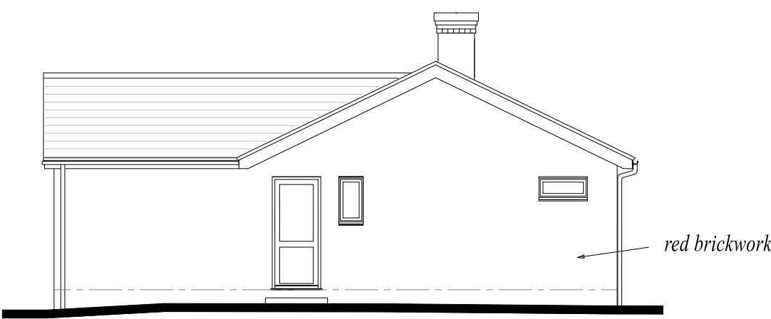
SIDE ELEVATION
