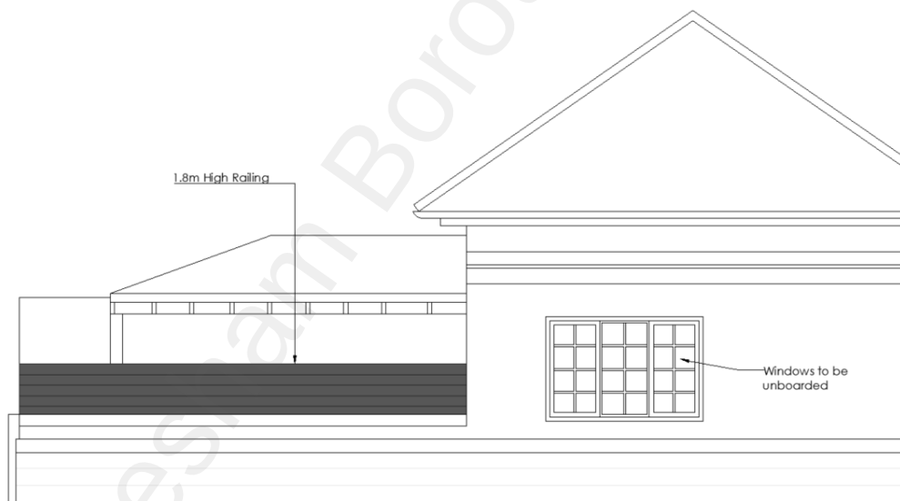
SIDE ELEVATION
