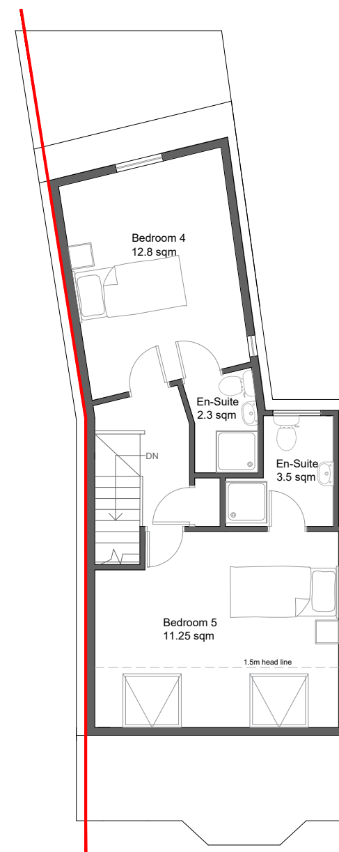
Existing/Proposed Loft Floor Plan
