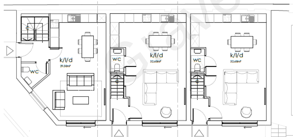
NEW BUILD: Ground Floor Proposed Plan
