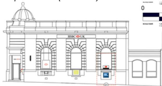
Proposed North (New Road) Elevation
