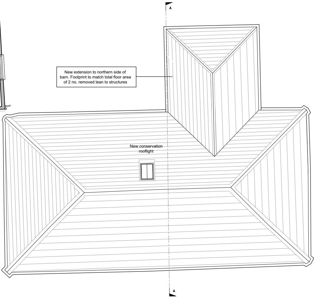
Proposed Roof Plan Scale 1:100 @ A3
