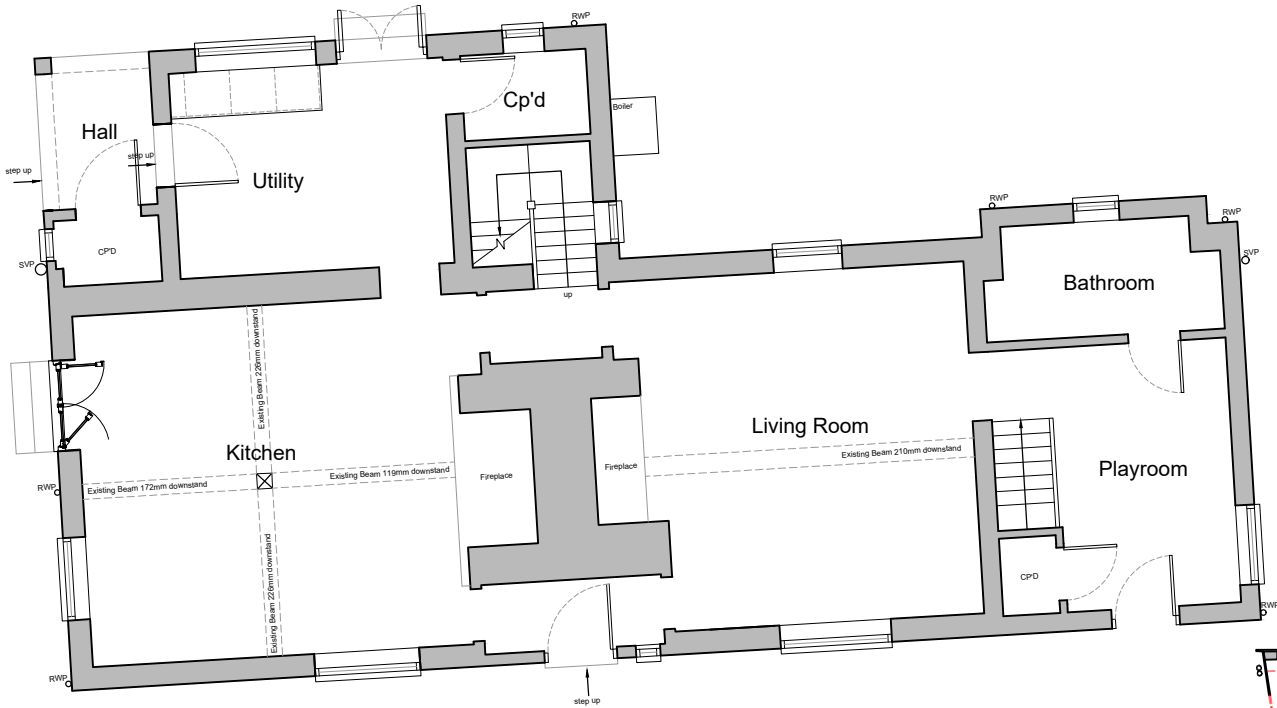
Demolition Ground Floor Plan Scale 1:100 @ A3
