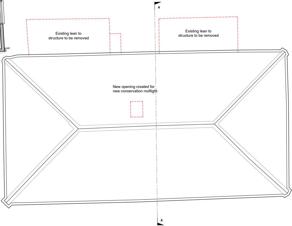
Demolition Roof Plan Scale 1:100 @ A3
