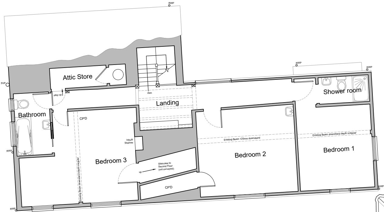
Demolition First Floor Plan Scale 1:100 @ A3
