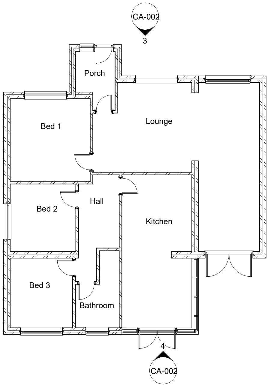
1 Ground Floor Plan 1 : 100
