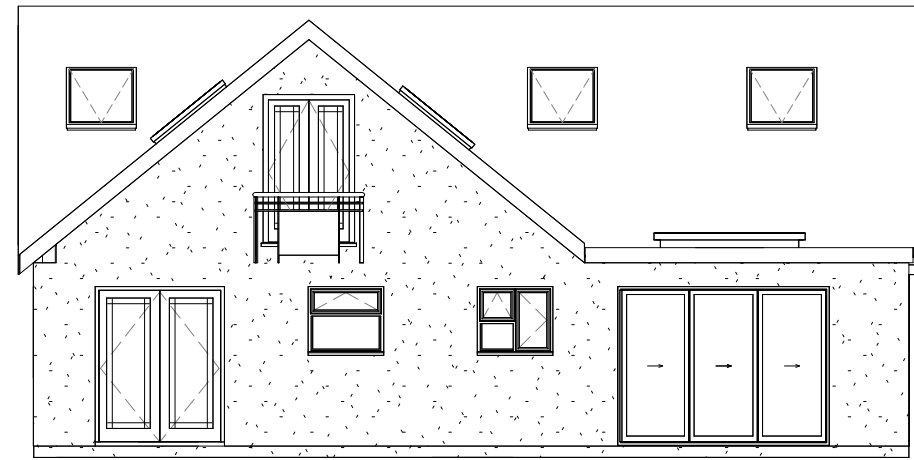
4 Rear Elevation 1 : 100
