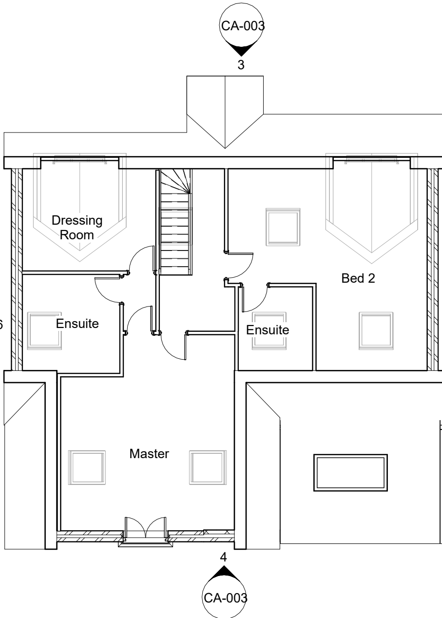
7 First Floor 1 : 100
