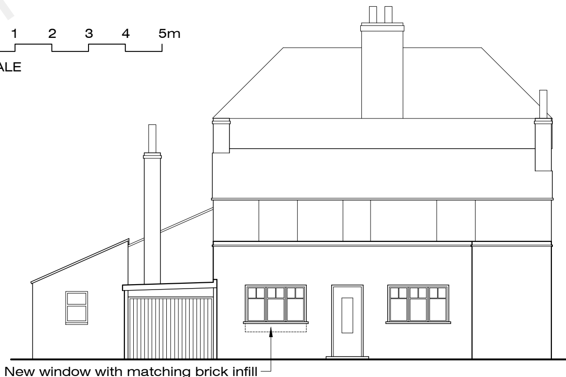
Proposed N (Rear Elevation)
