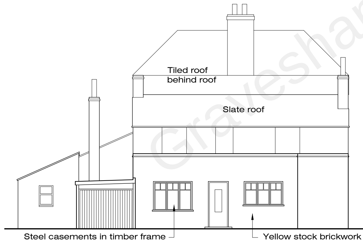
Existing N (Rear) Elevation
