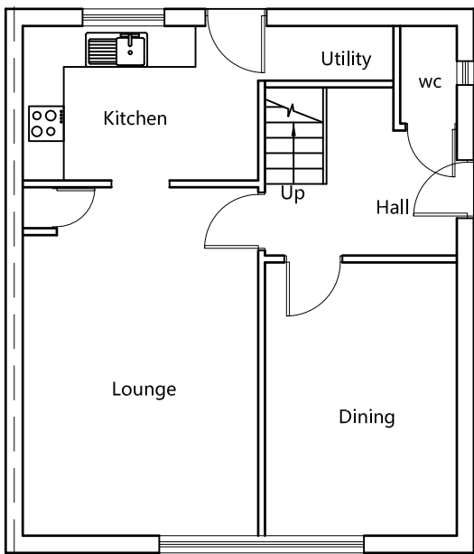
Pre-Existing Ground Floor Plan
