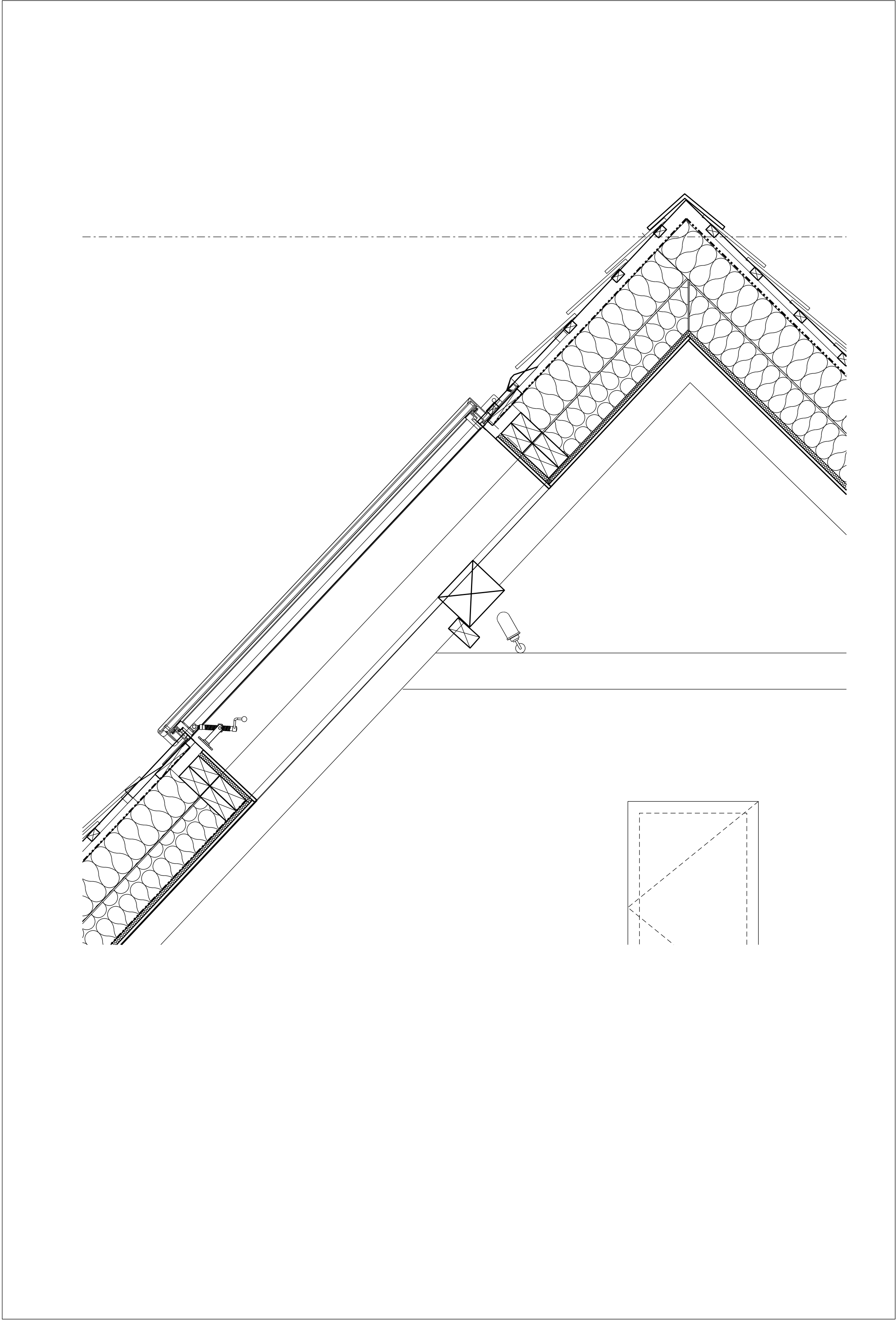
DETAIL - GF.W.01
