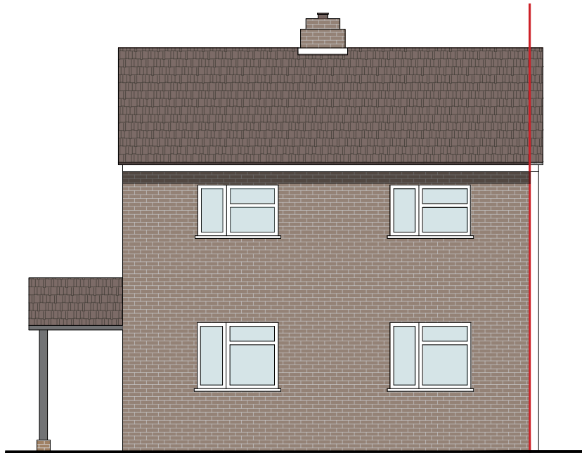
West Side Elevation
