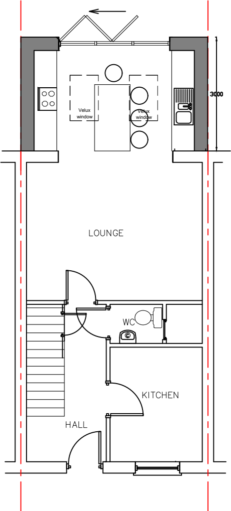
GROUND FLOOR PLANS
